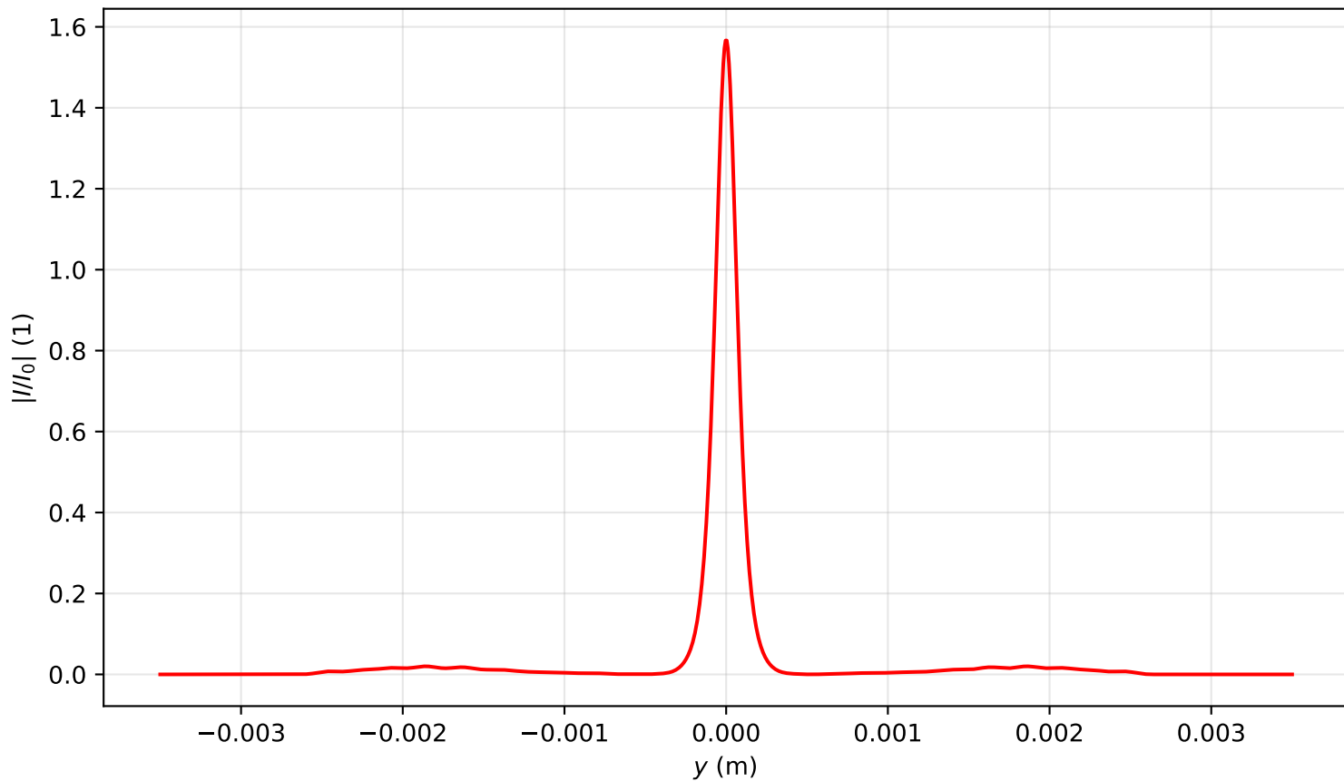
Intensity profile I(x=0, y, z=1.592)/I_0 , P_{in}=8.0P_{cr} , artificial time
